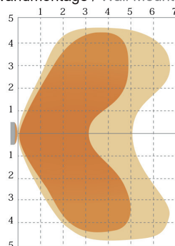
Wandmontage / Wall Mounted
